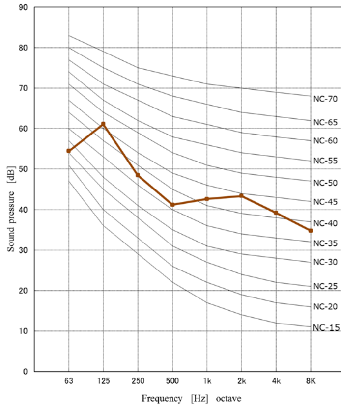
NC curves
